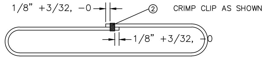
ZM-1 upper shock cord, cord length 21"
